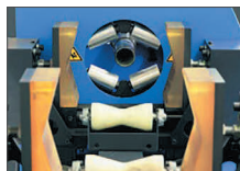
Clamping and guiding unit with wheels for up to 5"-hoses.
